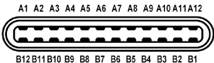
Figura 12. Puerto USB-C
