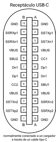
Figura 9. Puerto USB-C
